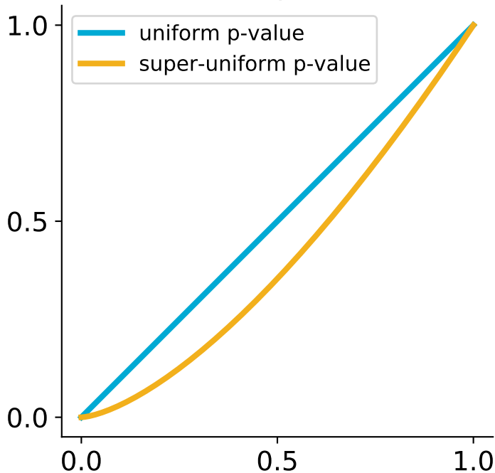
CDFs of p-values
